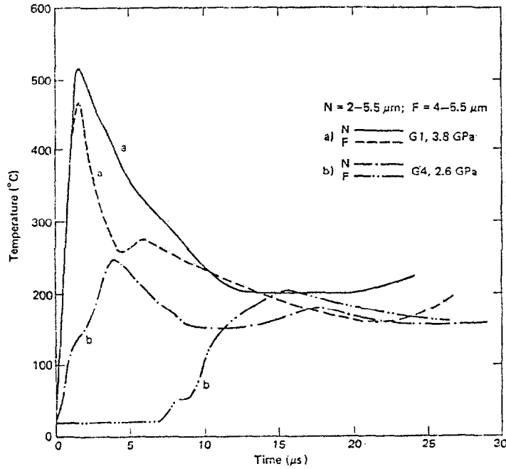
Fig 21 Blackbody Temperature - Time Plots For Two Bare Charge Shots
